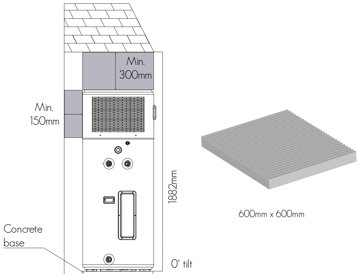
Figure 1: Side profile installation requirements and an example concrete base.
